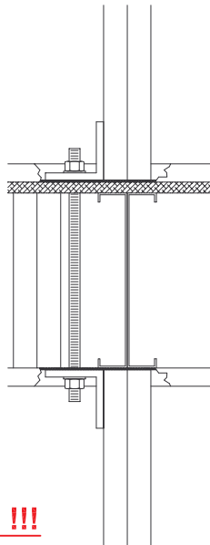
VIEW "1"
